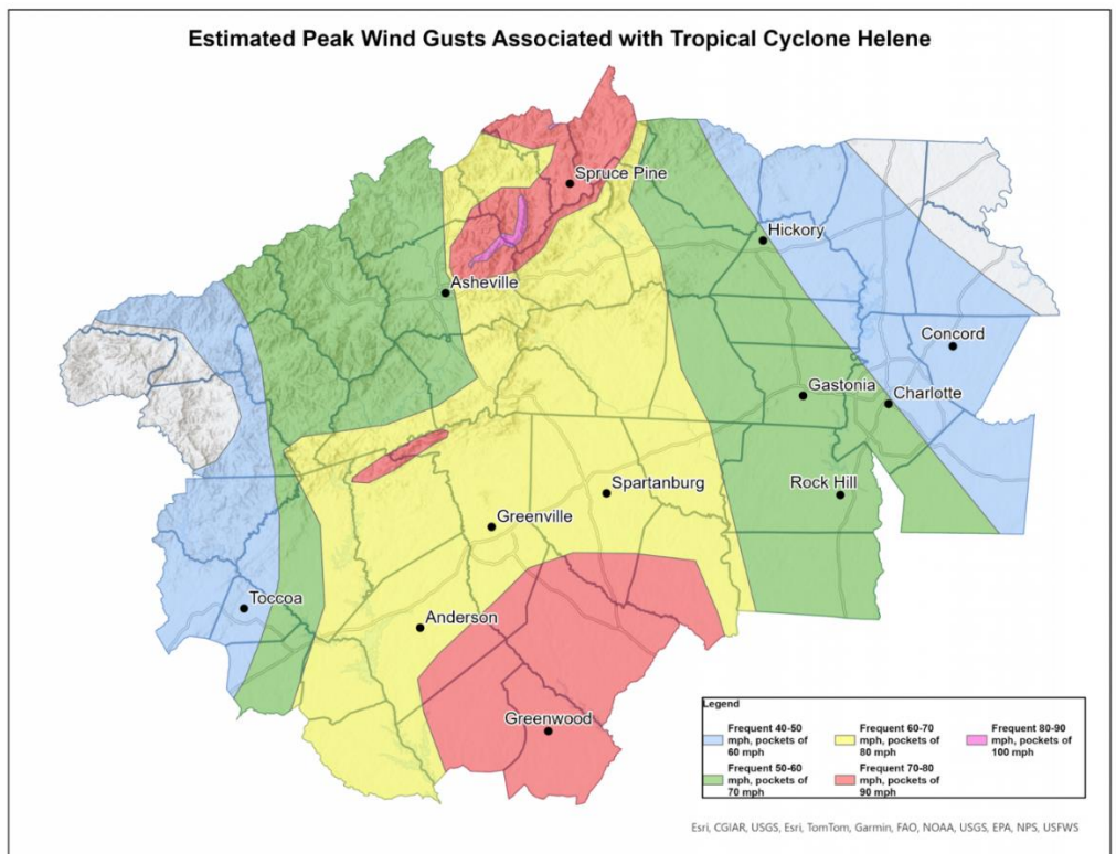
Figure 6: Estimated Peak Wind Gusts from Helene
