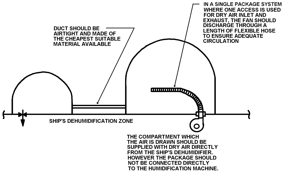
Figure 050-6-4. Ship Zone Dehumidification
