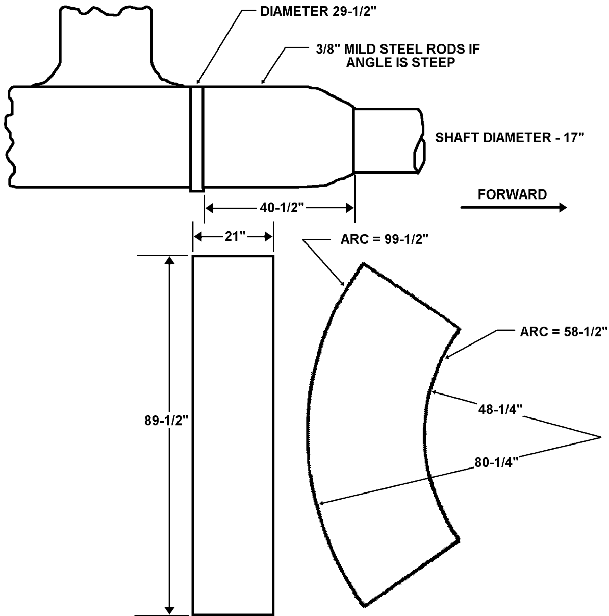
Figure 050-3-6 Double-Boot Method
