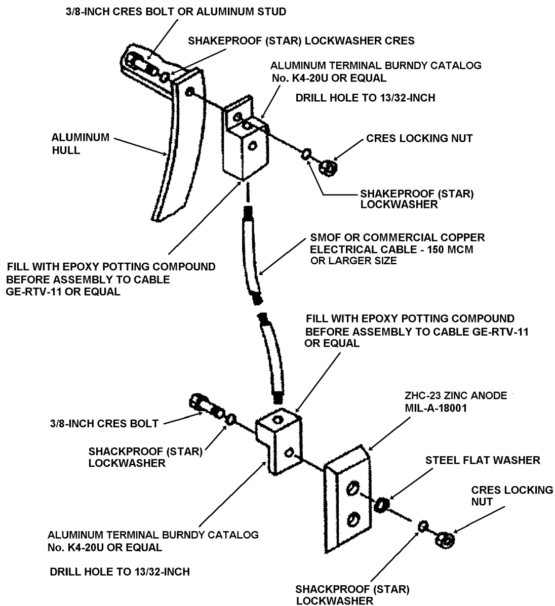
Figure 050-5-13. Anode Suspension, Aluminum Hull, Salt Water
