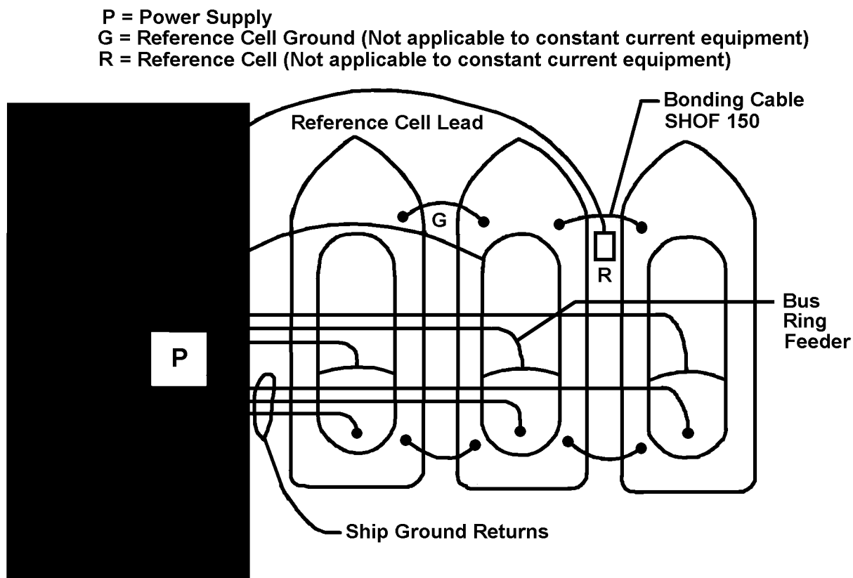
Figure 050-5-10. Automatic Control Equipment, Nest Installation
