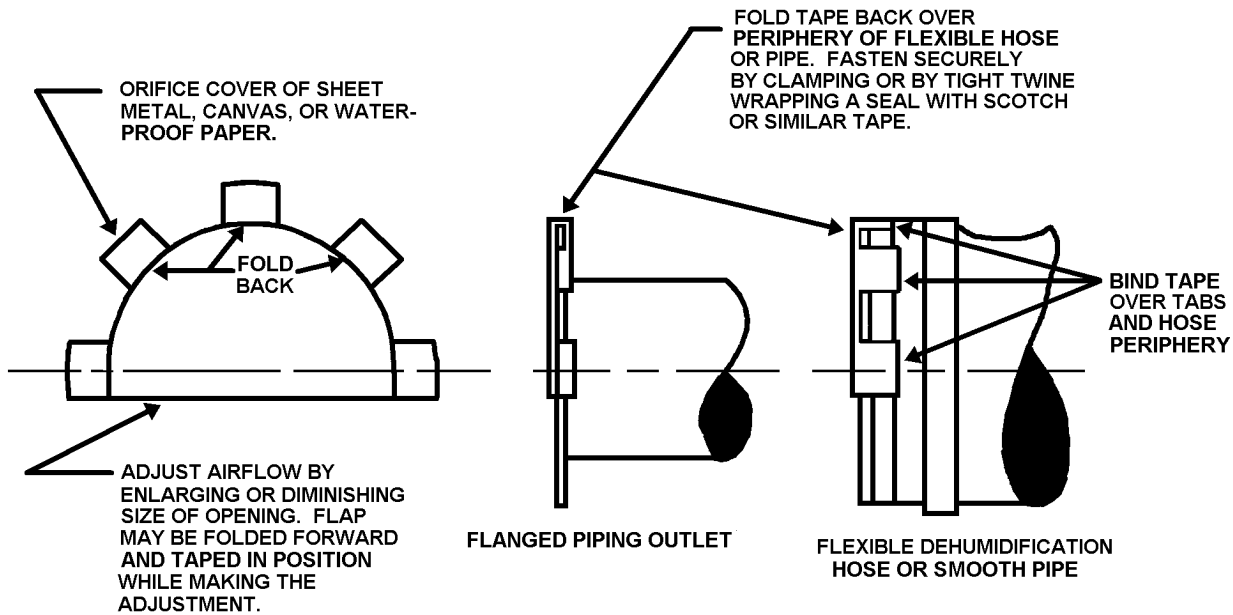
Figure 050-6-1. Throttling Device
