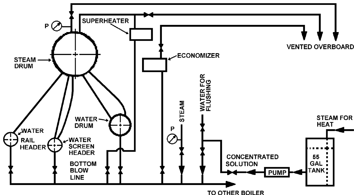
Figure 050-11-3. Boiler Boil-Out
